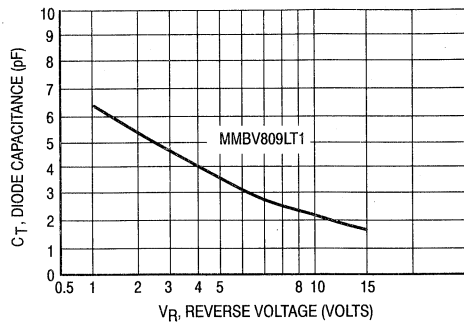
Figure 4. Diode Capacitance
