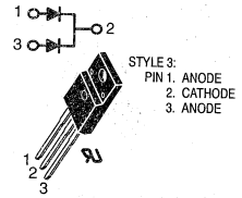
Case 221D
