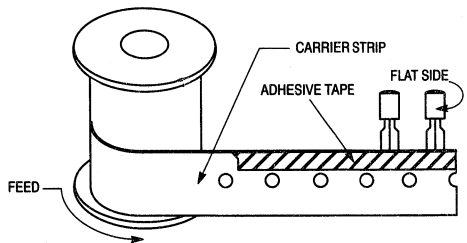
Figure 11. Style E
