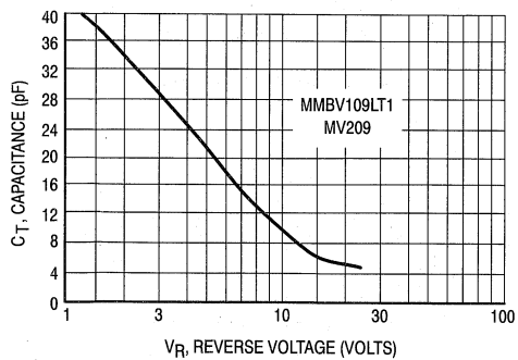
Figure 2. Diode Capacitance
