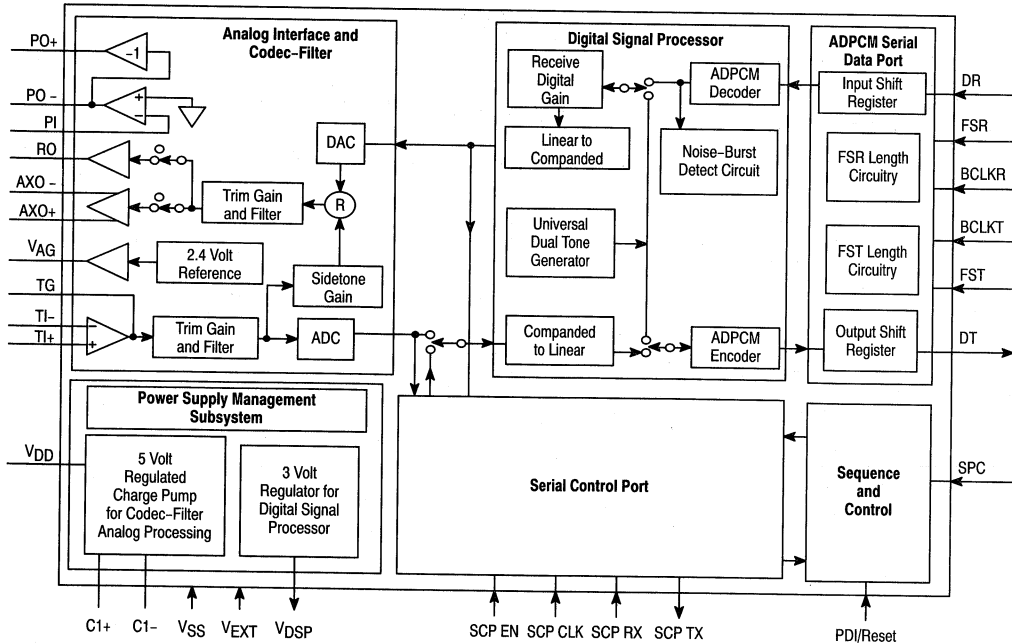
Figure 21. MC145540 ADPCM Codec Block Diagram
