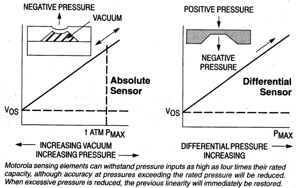
Figure 3. Pressure Measurements
