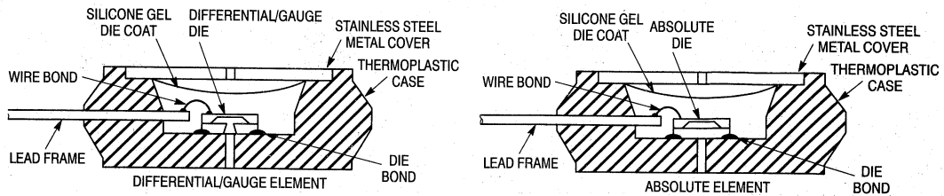
Figure 8. Cross-Sectional Diagrams (not to scale)
