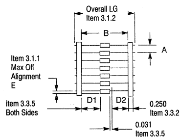
Figure 2. Component Spacing
