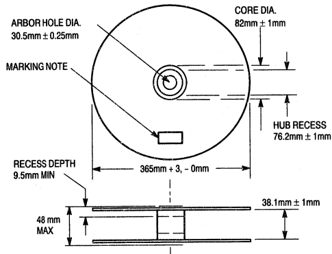
Figure 8. Reel Specifications
