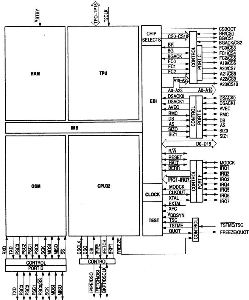
Figure 13. MC68332 Block Diagram
