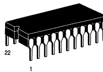
J SUFFIX CERAMIC CASE 736-05
