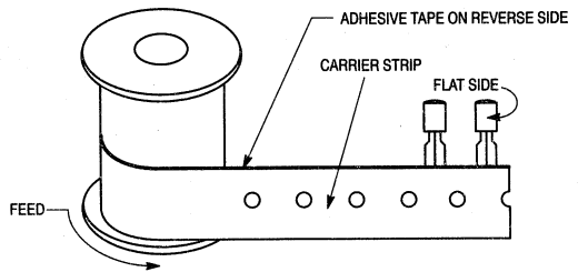
Figure 8. Reel Specifications
