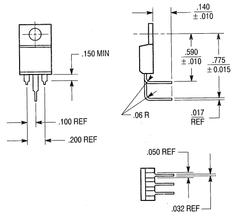
LEADFORM AK
