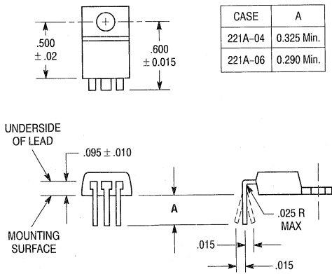
LEADFORM BL
