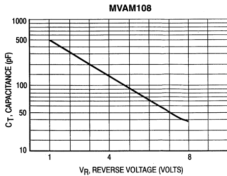
Figure 7. Capacitance versus Reverse Voltage
