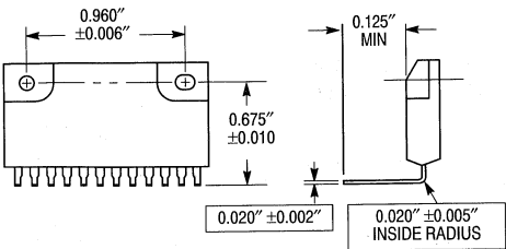
Leadform A
