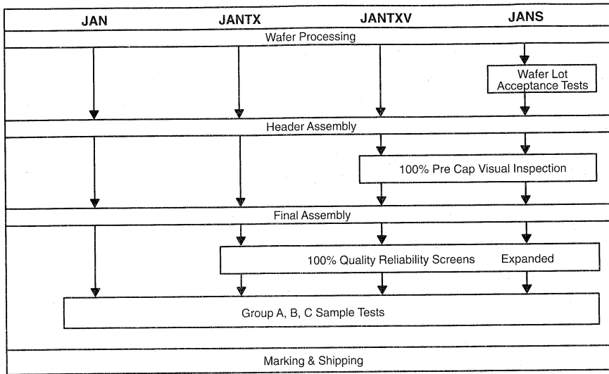
Figure 1. The MIL-S-19500 Semiconductor Process Flow
