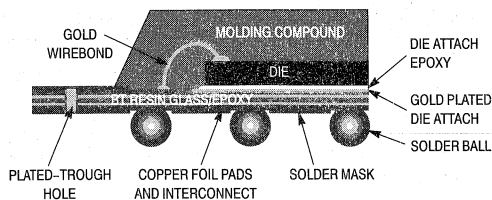
Figure 11. Simplified Cross-Sectional View of OMPAC
