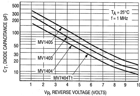
Figure 11. Diode Capacitance versus Reverse Voltage
