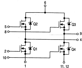
H-Bridge MPM3017
