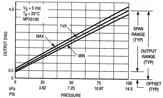
Figure 5. Signal Conditioned MPX5100
