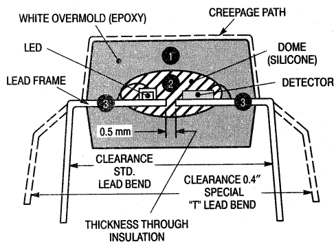
Figure 3. "DOME" Package
