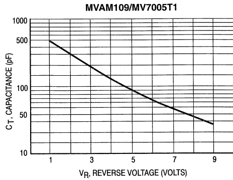
Figure 8. Capacitance versus Reverse Voltage
