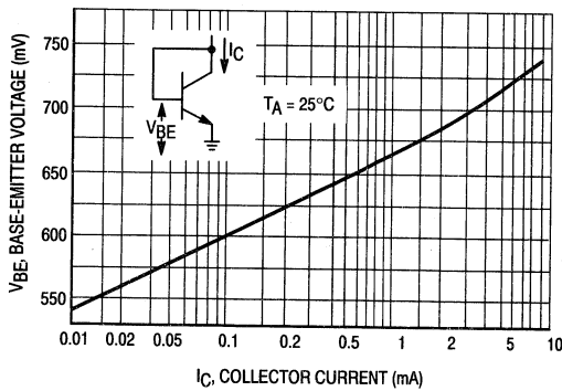
Figure 1. Base-Emitter Voltage versus Collector-Emitter Current
