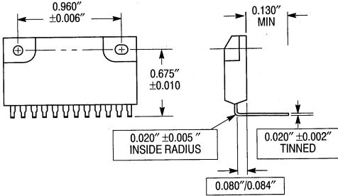
Leadform B
