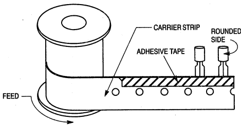
Figure 9. Style A
