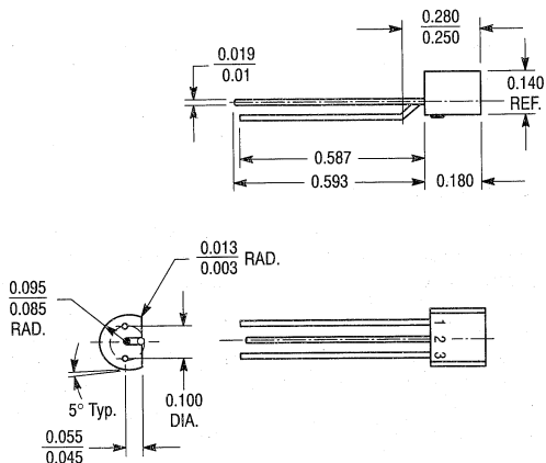
CASE 77 LEADFORM VB
