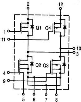
H-Bridge with Current Sensing MPM3002/MPM3010
