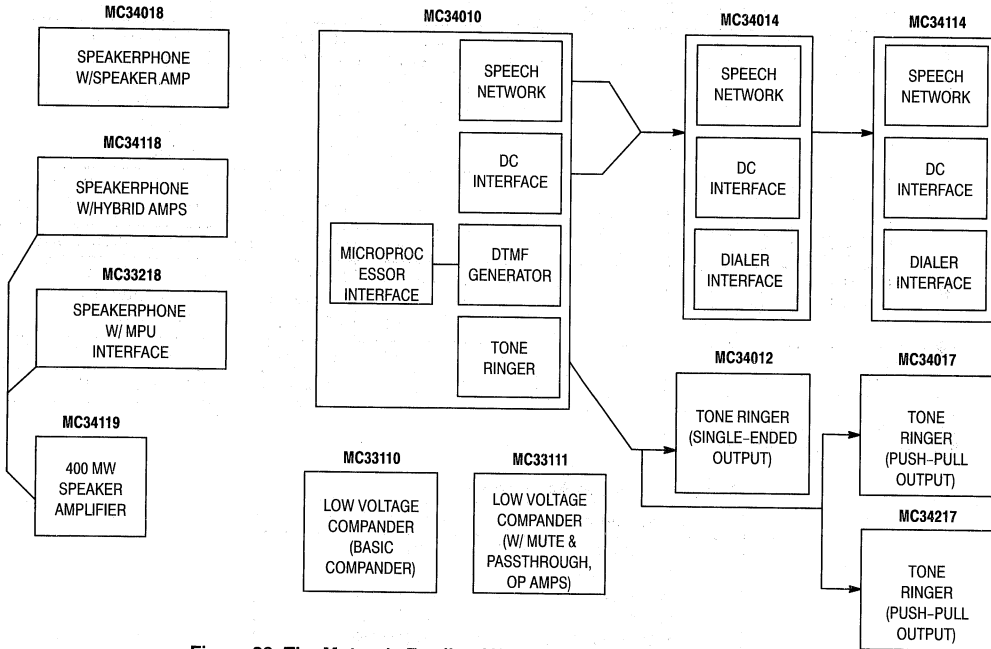
Figure 23. The Motorola Family of Handset Telecom Integrated Circuits
