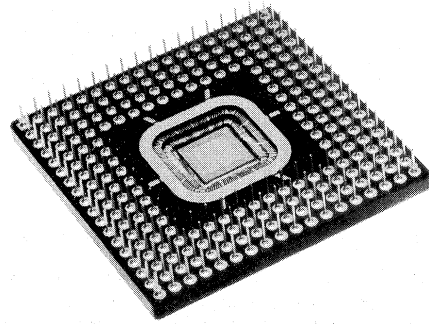
Figure 1. MCA6200ETL in Multi-Layer Ceramic 224 Pin-Grid-Array Designed for High Frequency, Mixed-Mode Applications
