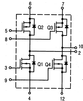
H-Bridge MPM3004
