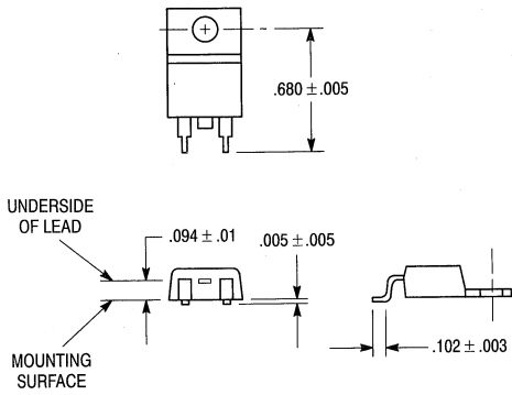
LEADFORM BD
