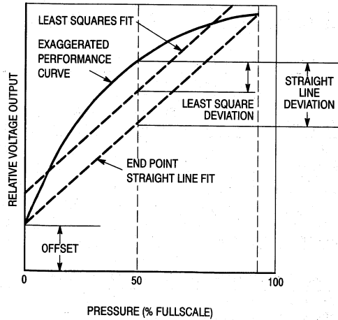
Figure 2. Linearity Specification Comparison
