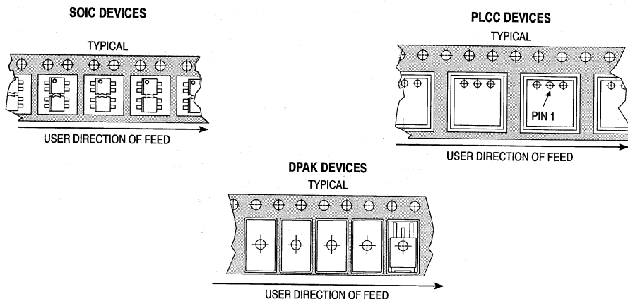
Figure 5. Mechanical Polarization
