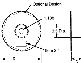
Figure 3. Reel Dimensions
