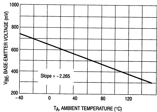
Figure 2. Base-Emitter Voltage versus Ambient Temperature
